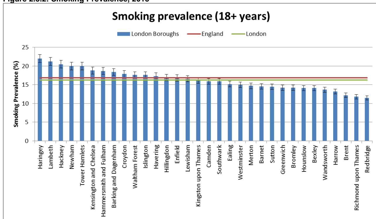
Figure 2.5.2: Smoking Prevalence, 2015
